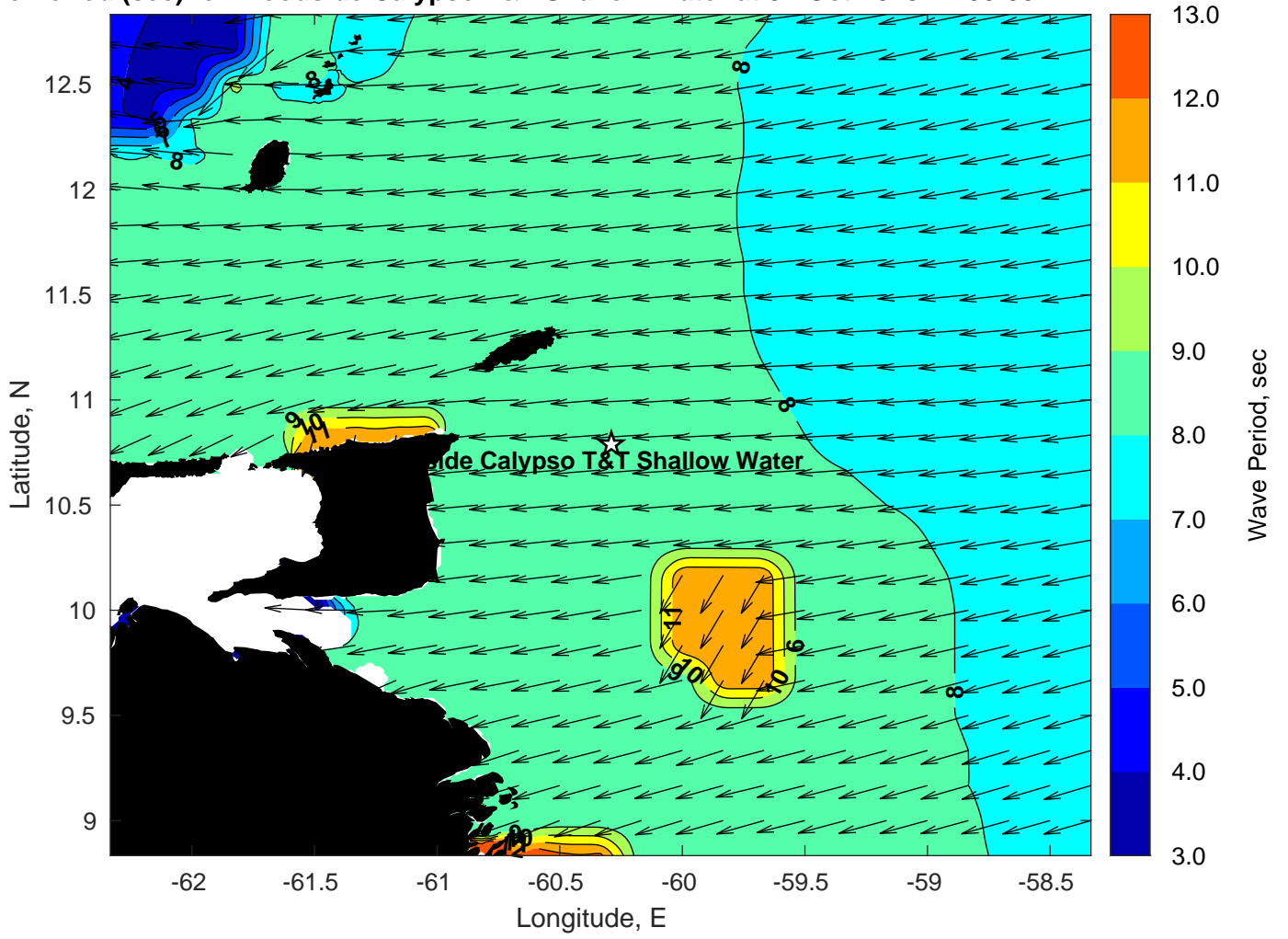
Wave Period (sec) for Woodside Calypso T&T Shallow Water at 31-Oct-2023 12:00:00
